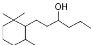
Cyclohexanepropanol, 2,2,6-trimethyl-, alpha.-propyl-
